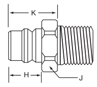
Male Pipe Thread
